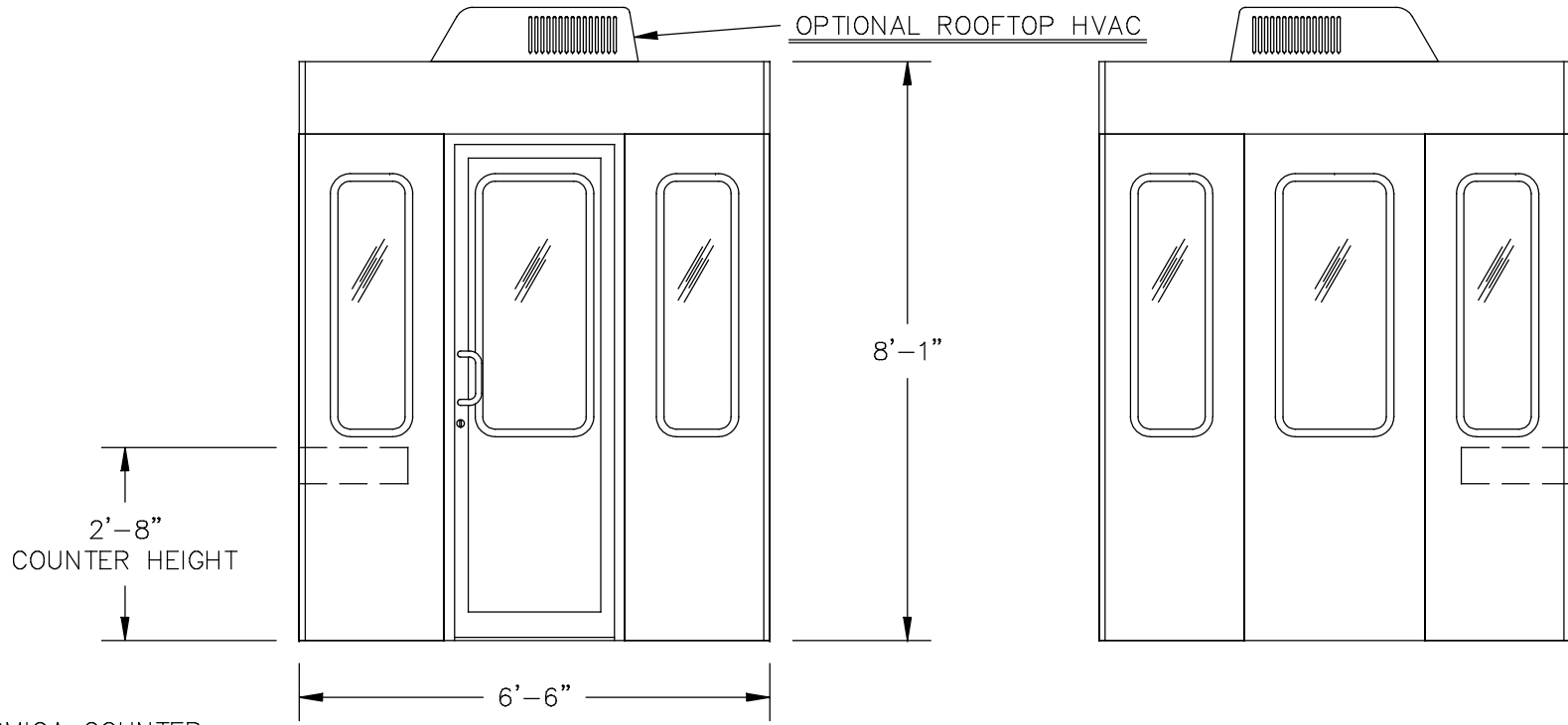
SIDE ELEVATION
