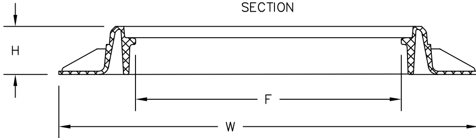
SECTION VIEW COVER REMOVED FOR CLARITY
