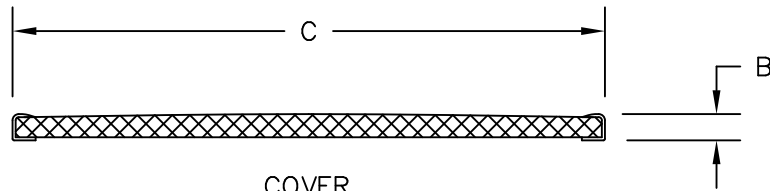
COVER SECTION
